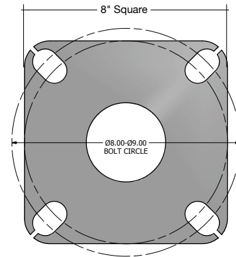
8" X 8" X .75" THICK BASE PLATE
