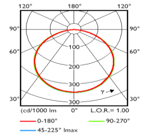
Photometric Curv
