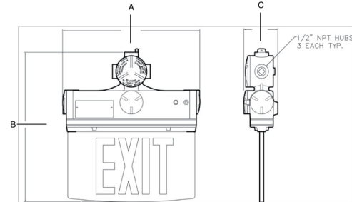
EHLEX Series Fixture Dimensions (inches)
